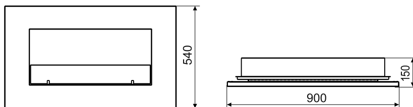
Built-in
